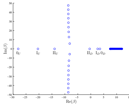
Figure 2. Values of \beta in complex plane.
