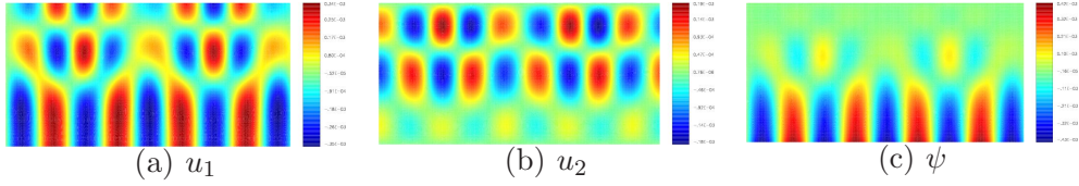
Figure 3. Isovalues of the real part of the components of the computed displacement field and vorticity (combination A).
