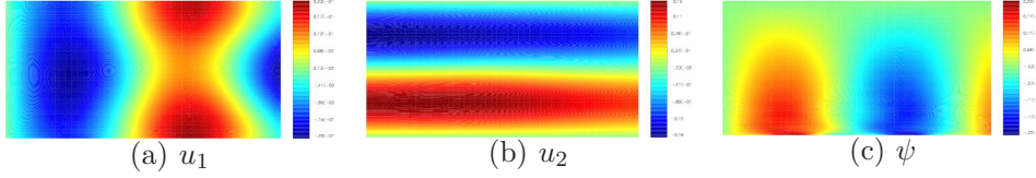
Figure 4. Isovalues of the real part of the components of the computed displacement field and vorticity (combination B).
