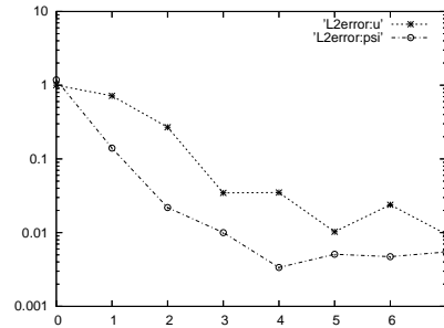
Figure 5. Behavior of the logarithm of the relative L^2 error in \mathbf{u} and \psi .
