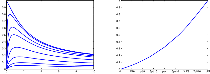
Figure 2: Left : graph of function k_\theta for increasing values of \theta : \pi/16, \pi/10, \pi/6, \pi/4, \pi/3, 3\pi/8, 7\pi/16, \pi/2 . Right : function \kappa_0(\theta)
