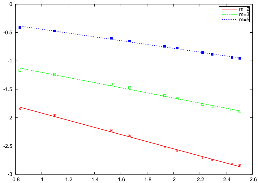
Figure 5: Function F for 2\theta = \pi/3 and m = 2, 3, 5
